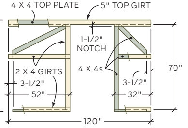
FRONT WALL
