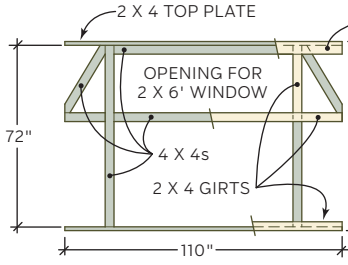
REAR WALL
