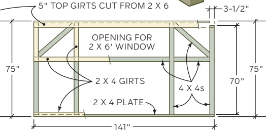
SIDE WALL
